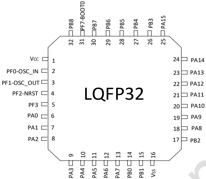
图 3-5 LQFP32 Pinout1 PY32F031K1xT6 (Top view)
