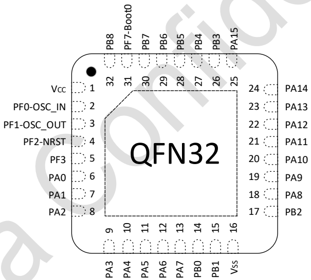
图 3-6 QFN32(5*5) Pinout1 PY32F031K1xU6 (Top view)
