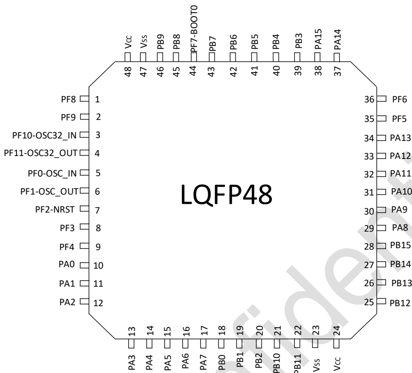
图 3-1 LQFP48 Pinout1 PY32F031C1xTx (Top view)
