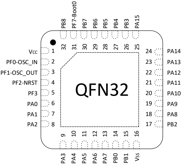
图 3-7 QFN32(4*4) Pinout2 PY32F031K2xU7 (Top view)
